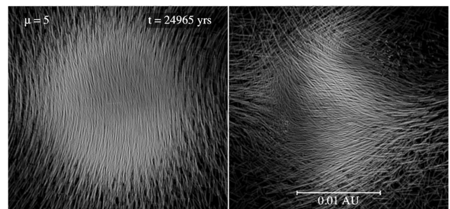
Figure 19. Magnetic field (left) and current density (right) in the stellar core from the \mu = 5 calculation, shown 0.2 yr after the formation of the stellar core. The magnetic field geometry in the stellar core is mainly poloidal (left-hand panel), consistent with the field being entrained in the stellar core from larger scales. The maximum field strength in the stellar core at this stage is \sim 30 kG.
