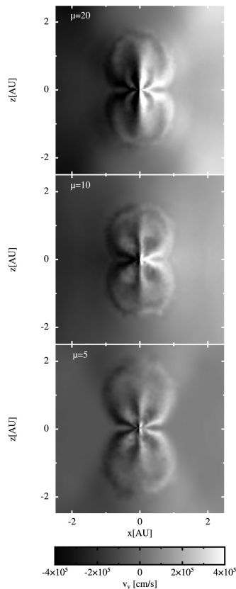
Figure 12. The velocity perpendicular to a slice through the outflow from the stellar core (i.e. v_{\perp} ) for each of the magnetized calculations that produces a stellar outflow, 1 yr after stellar-core formation in each case. As with the outflows from the first cores, the stellar outflows are clearly rotating in the same sense as the progenitor dense cores and the rotation rates are greater for calculations with lower initial magnetic field strengths. However, the rotation speeds are significantly lower than the outflow speeds.
