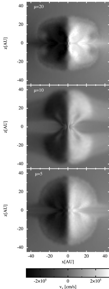
Figure 7. The velocity perpendicular to a slice through the outflow from the first hydrostatic core (i.e. v_y ) for each of the magnetized calculations that produces an outflow, just before each calculation forms a stellar core. The outflows are clearly rotating in the same sense as the progenitor dense cores, with rotation speeds that are similar to the outflow speeds.
