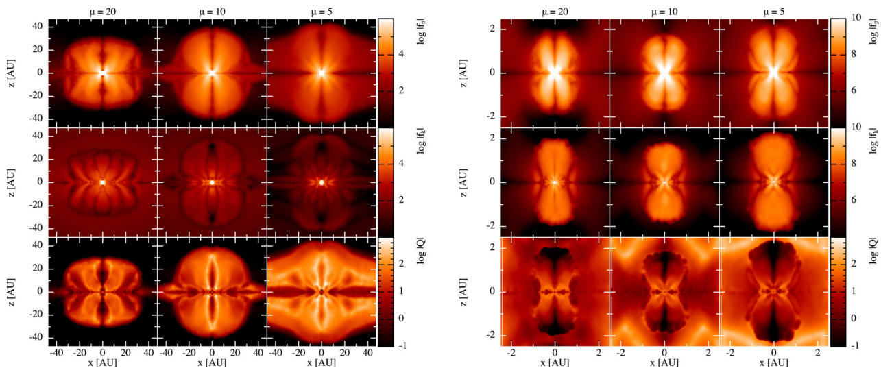
Figure 18. Cross-sections of the magnitude of the vertical component of the Poynting flux f_p (top row), magnitude of the vertical component of the kinetic flux f_k (second row), and their ratio Q (bottom row) in the outflows from the first core (left-hand panels) and the second core (right-hand panels). The plots are shown 1 yr after stellar-core formation in the calculations with initial mass-to-flux ratios of \mu = 20, 10 and 5 times critical (left to right). All the outflows are Poynting flux dominated away from the outflow axis. In the outflows from the first cores, the gas is actually infalling along much of the outflow axis. In the outflows from the stellar cores, the flow is outwards along the axis but the kinetic flux dominates over the Poynting flux.
