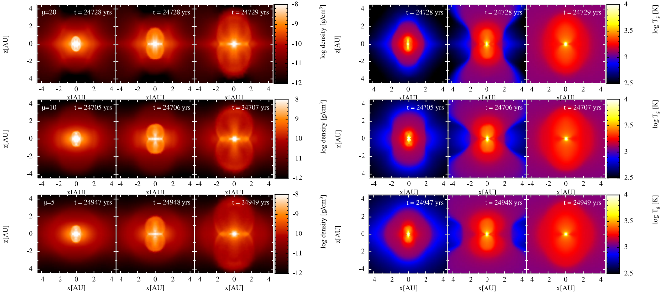
Figure 10. Snapshots of the density (left-hand panels) and temperature (right-hand panels) on slices parallel to the rotation axis showing the development of the outflows that are launched from the stellar cores in the three most magnetized calculations. From top to bottom, each row is for cloud cores with initial mass-to-flux ratios of \mu = 20, 10 and 5 times critical, respectively. For each case, we show snapshots 0.5, 1.0 and 2.0 yr after stellar-core formation. The structure of the stellar outflows is similar for each initial magnetic field strength, but it appears that weaker initial fields produce slightly better collimation. The remnants of the first hydrostatic cores are clearly visible in the density slices (thickness |z| \approx 3 au), and the stellar outflows are followed until just after they have broken out of the first core in each case.
