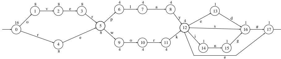
Figure 11: The numbered version of the automaton
