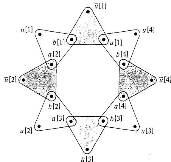
Figure 3.2 Truth setting component T_i when m = 4 (subscripts have been deleted for simplicity). Either all the sets of T_i^f (the shaded sets) or all the sets of T_i (the unshaded sets) must be chosen, leaving uncovered all the u_i[j] or all the \bar{u}_i[j] , respectively.
