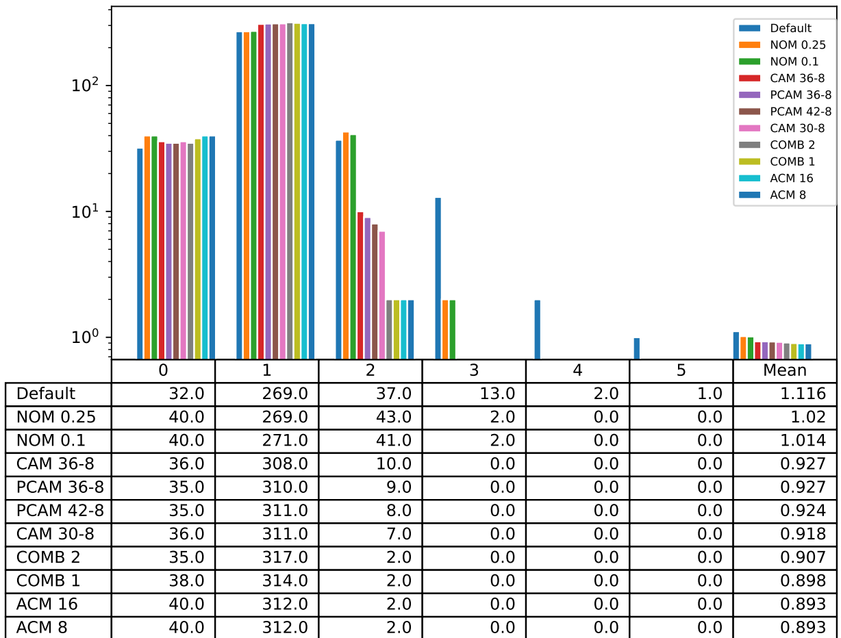
Figure 5.13: Number of jumps performed per-search across all searches
