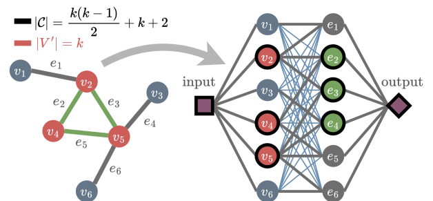
Figure 2: Schematic of the reduction from CLIQUE (left).
