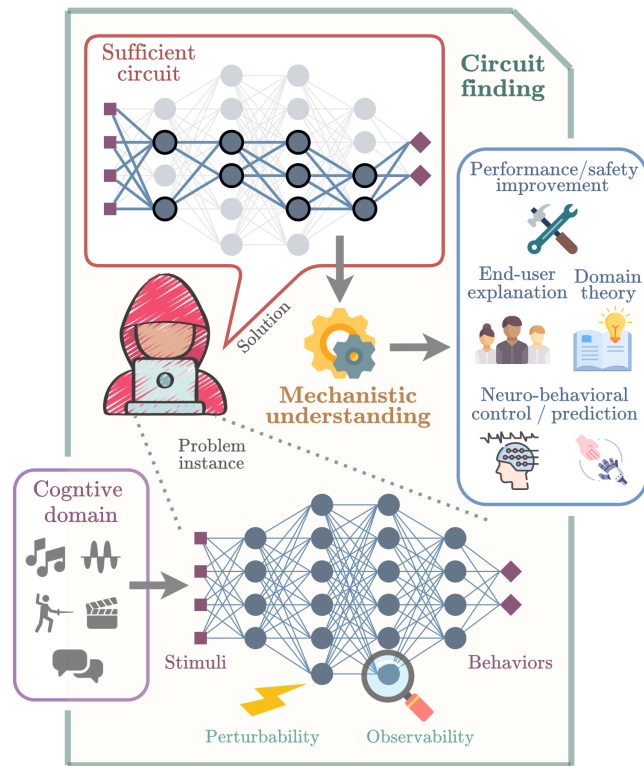
Figure 1: Schematic of the problem of reverse-engineering neural networks (bottom) trained in a domain of interest (left), the interpretability task of circuit finding (top), and its intended application in various disciplines (right).
