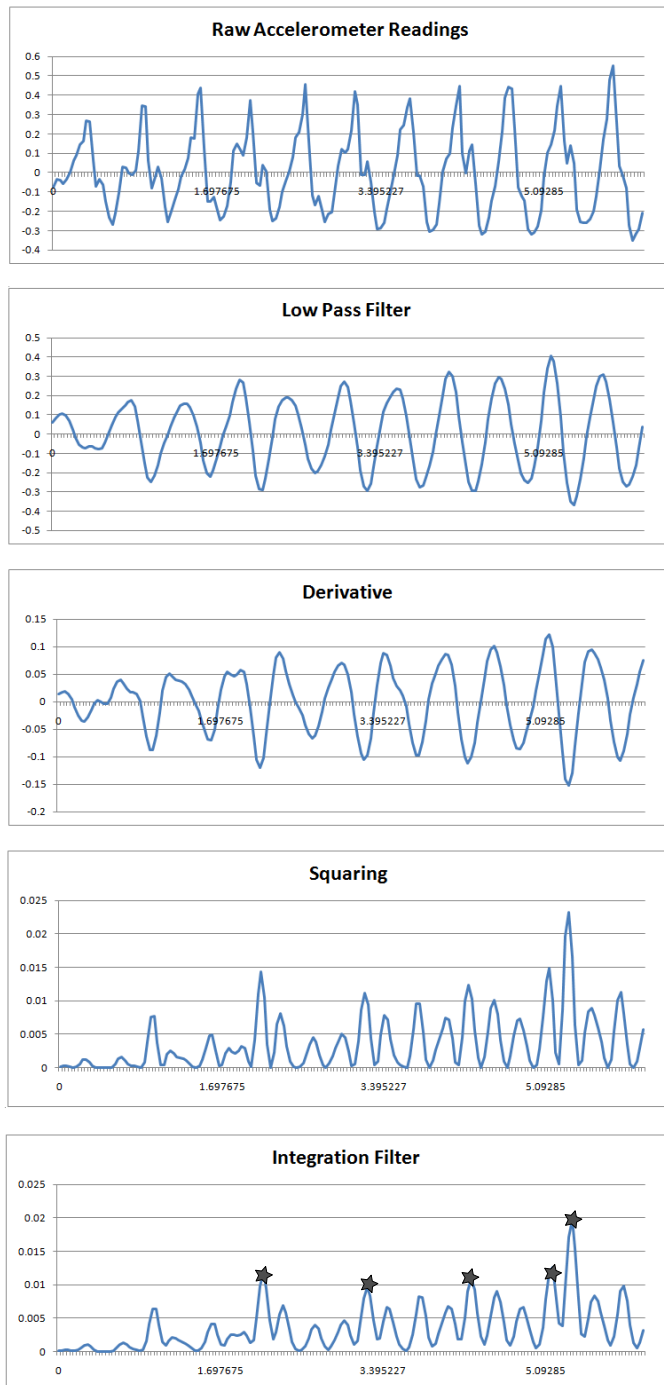
Figure 3.9: Results of the Pan-Tomkins method on the magnitude acceleration for 6 seconds. The data was collect by walking in a straight path. Stars are showing the step detection.
