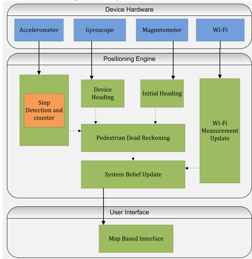
Figure 5.2: System Architecture
