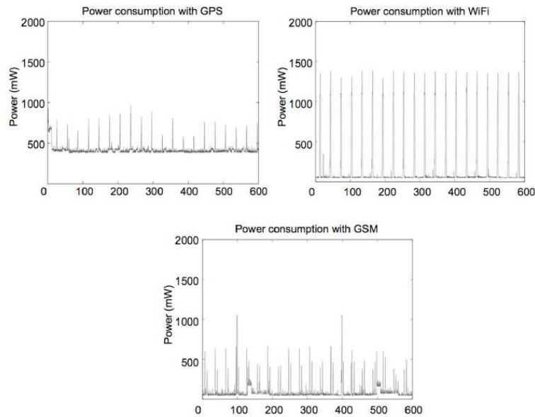
Figure 2.1: Power Consumption among different technologies [17]
