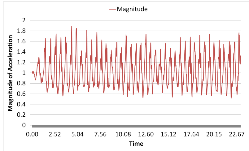
Figure 3.7: Magnitude of the accelerometer readings
