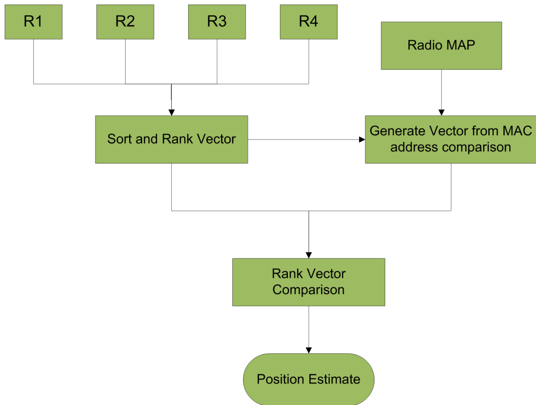
Figure 4.6: Block diagram for rank based fingerprinting algorithm
