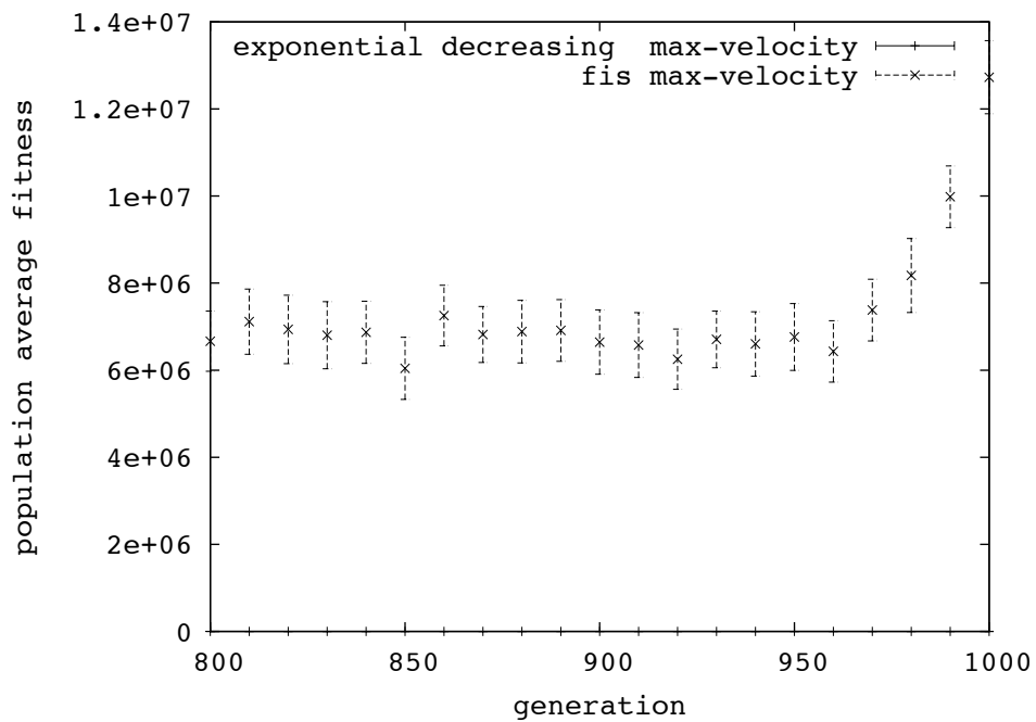
Figure 2: Average Population Fitness: last 200 generations.
