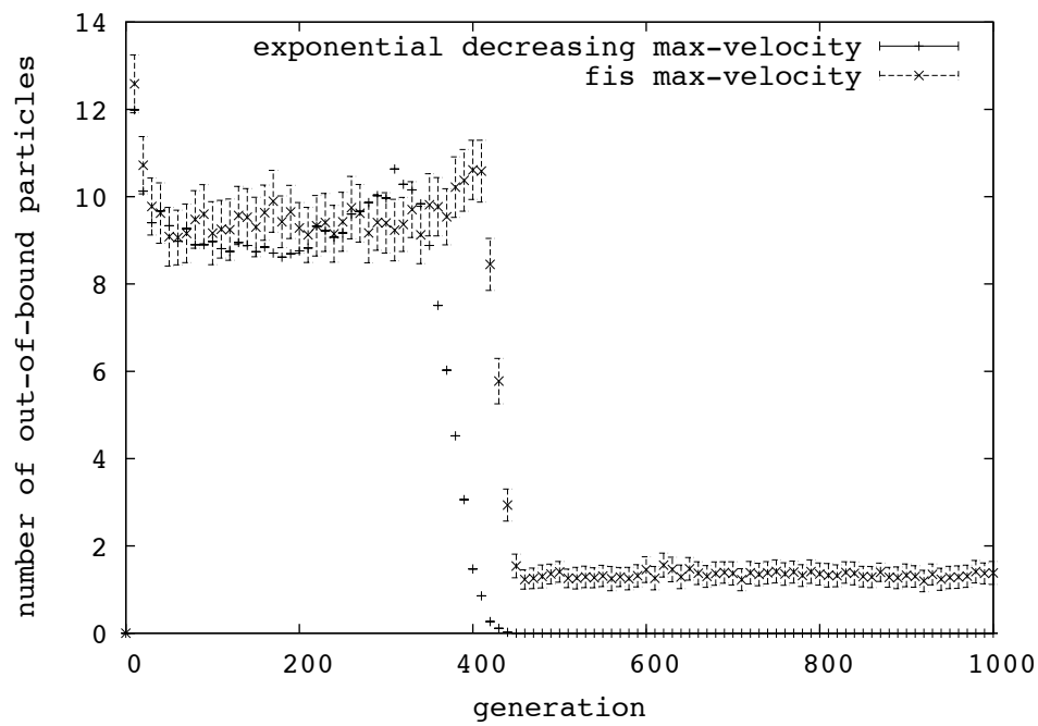
Figure 9: Average number of out-of-bound particles (dimension).
