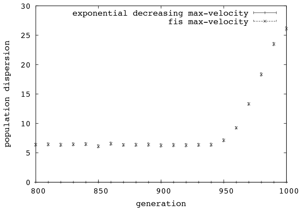
Figure 6: Population Dispersion: last 200 generations.
