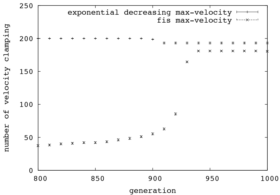
Figure 8: Average number of clamped particles (dimension: last 200 generations).
