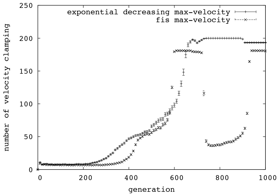
Figure 7: Average number of clamped particles (dimension).
