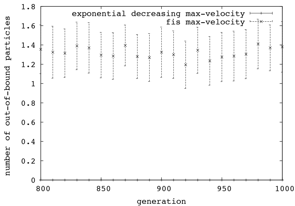
Figure 10: Average number of out-of-bound particles (dimension): last 200 generations.
