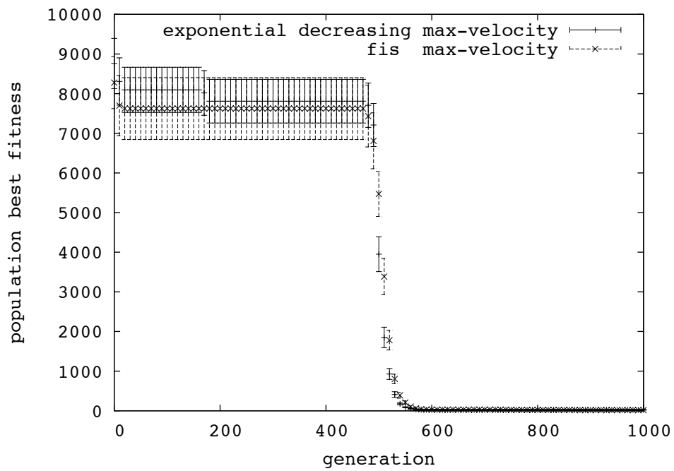
Figure 3: Population Best Fitness.
