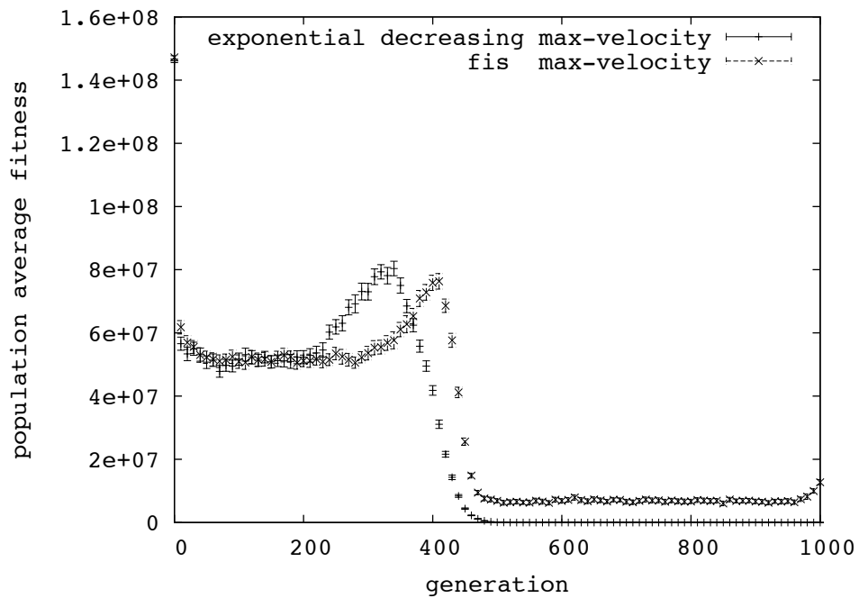
Figure 1: Population Average Fitness.
