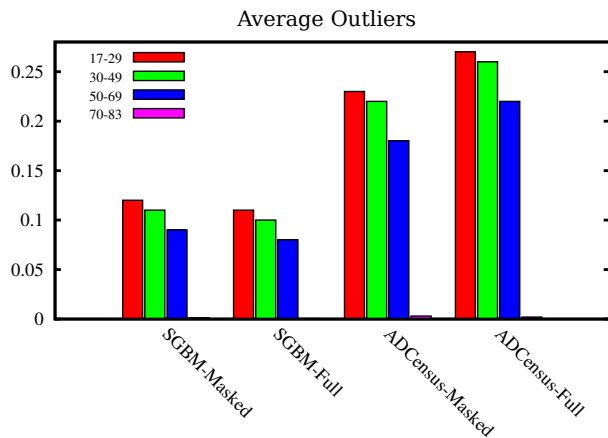
Figure 6: Average outliers for both SGBM and ADCensus
