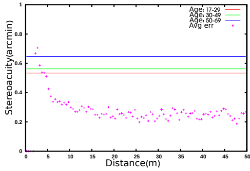
(a) Average relative depth error by SGBM
