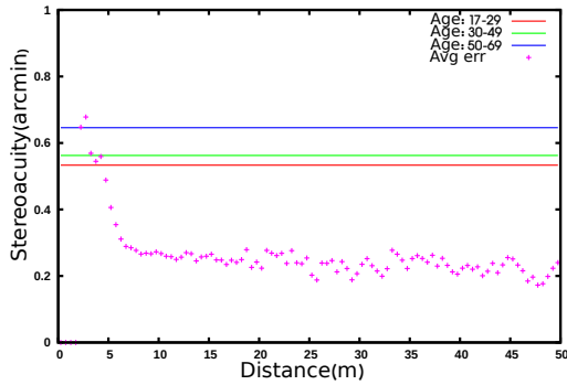
(a) Average relative depth error by SGBM
