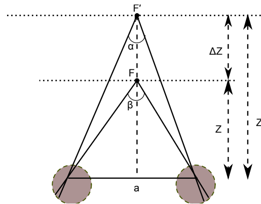
Figure 1: Binocular disparity
