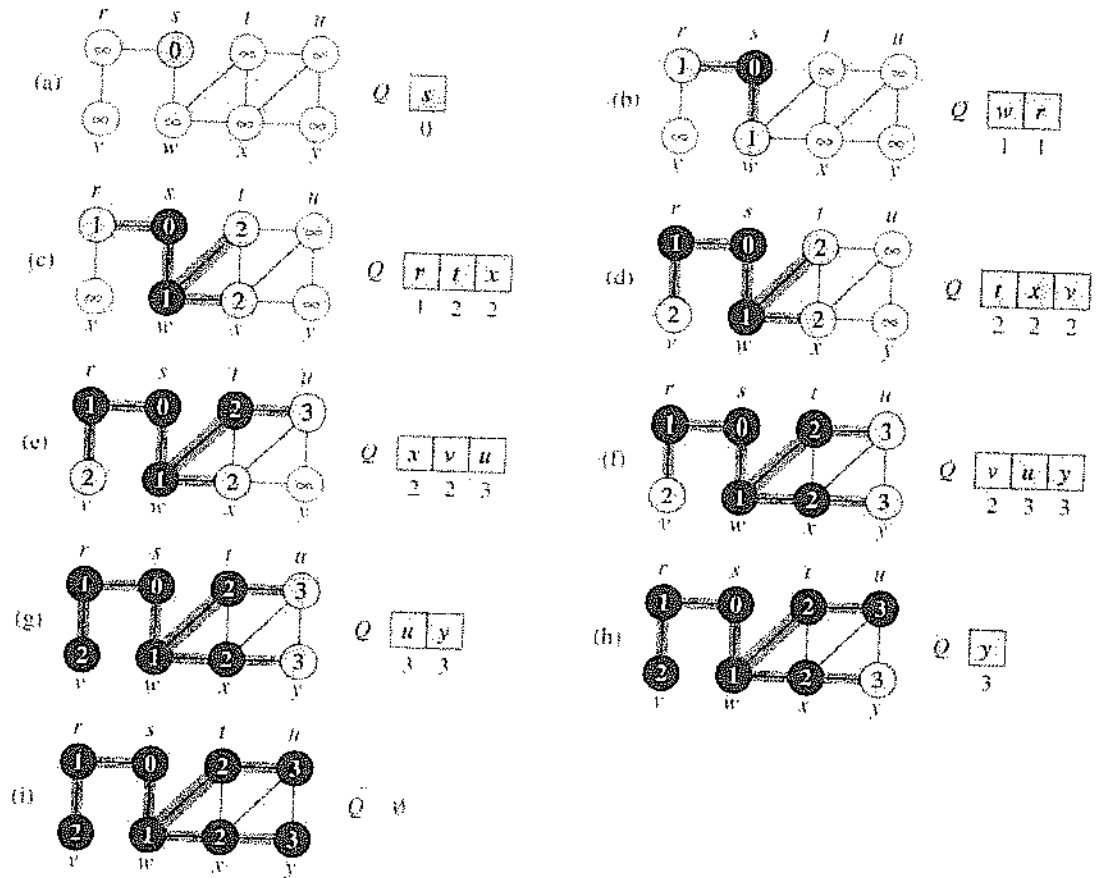
Figure 22.3 The operation of BFS on an undirected graph. Tree edges are shown shaded as they are produced by BFS. The value of u.d appears within each vertex u . The queue Q is shown at the beginning of each iteration of the while loop of lines 10–18. Vertex distances appear below vertices in the queue.
