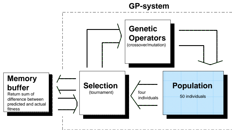
Figure 12: The memory based GP system in the learning process.
