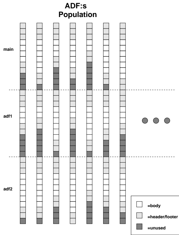
Figure 12.10 The structure of a population consisting of individuals with two ADF parts and a main part in AIM-GP
