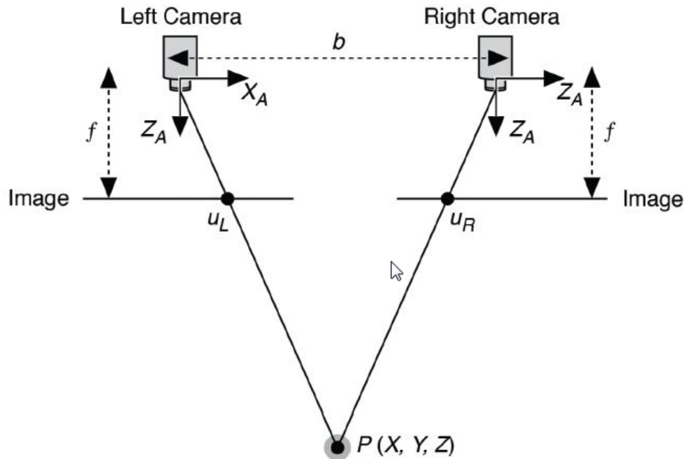
Figure 2.9: Stereo Vision
